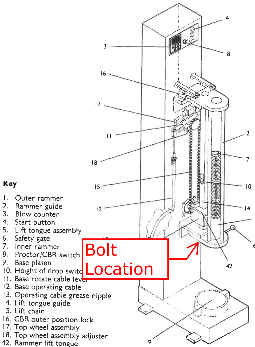
Figure 6 Automatic Compaction Machine (shown with guard completely removed exposing working parts to the operator)
