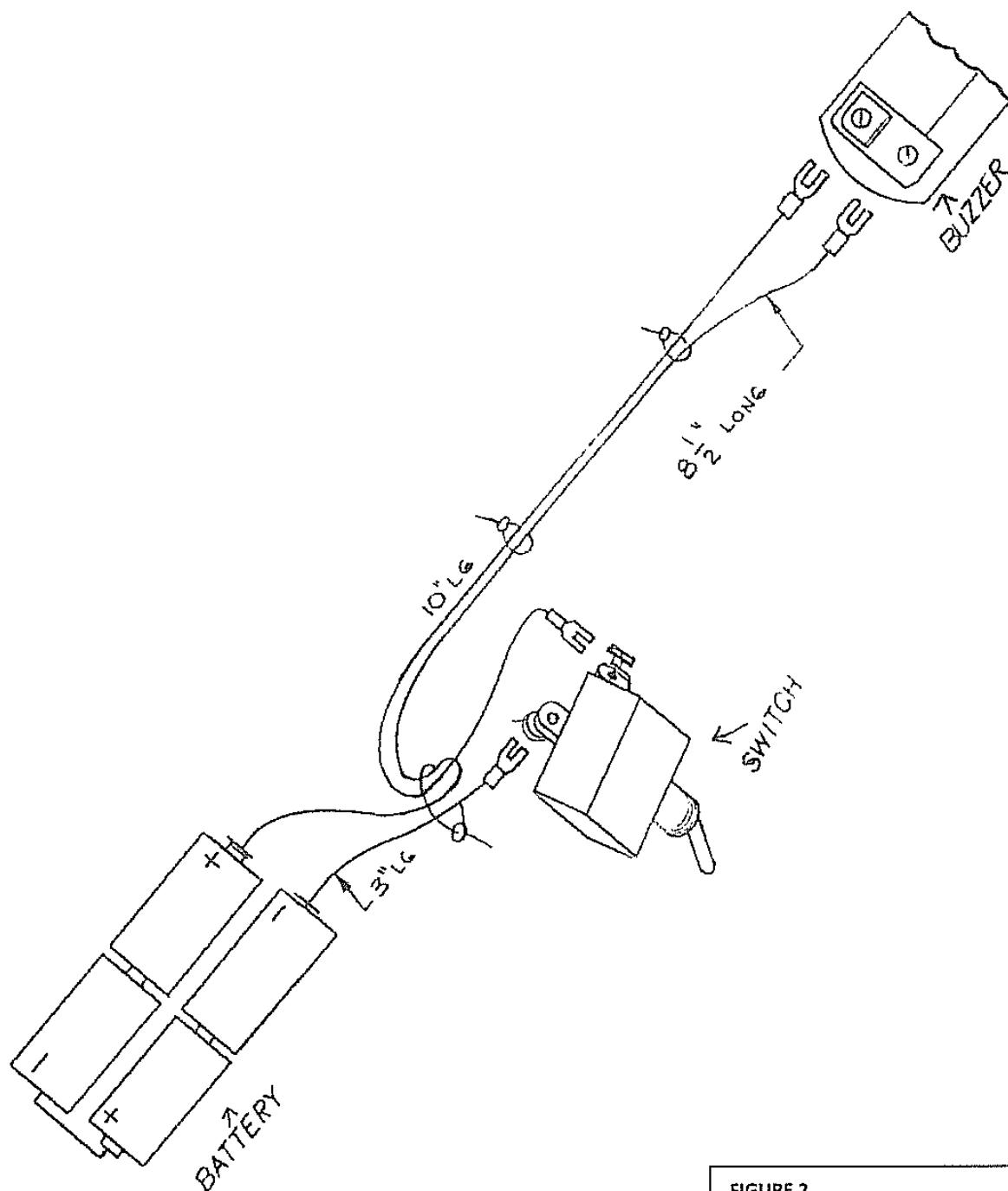
FIGURE 2 Battery Wiring Diagram
