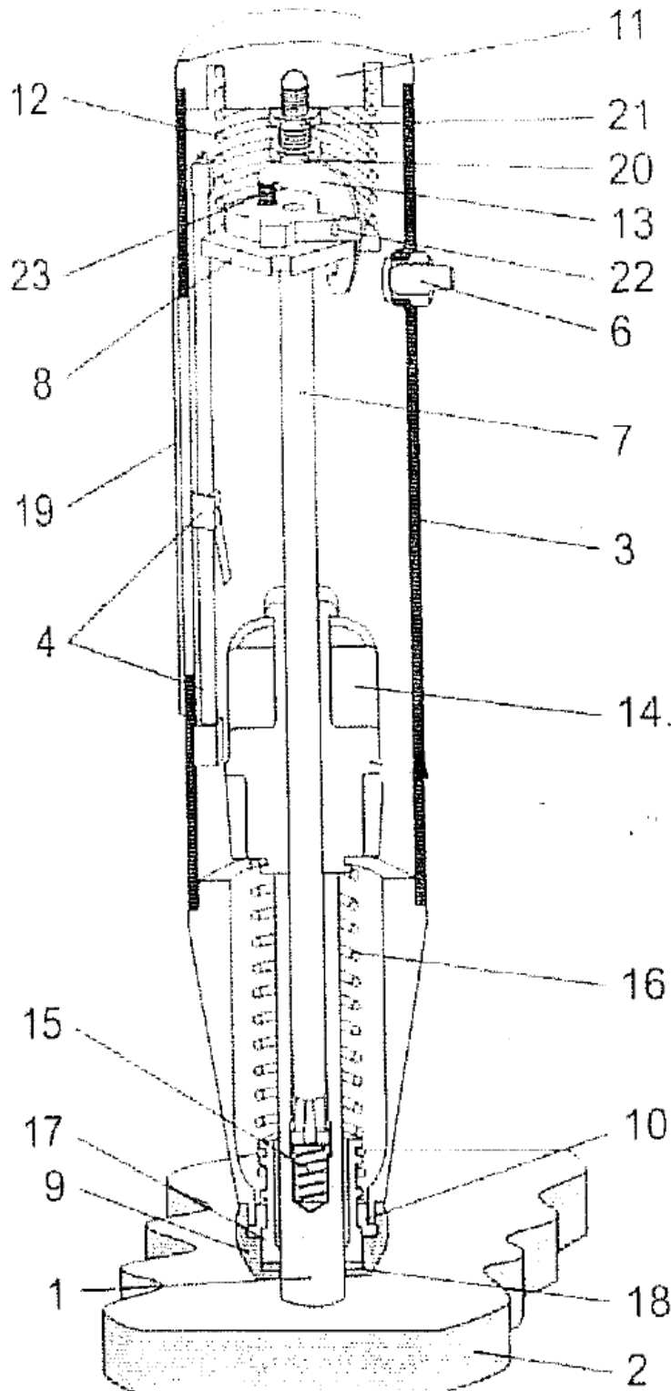
Figure 3.3 cross sectional cut through the concrete test hammer
