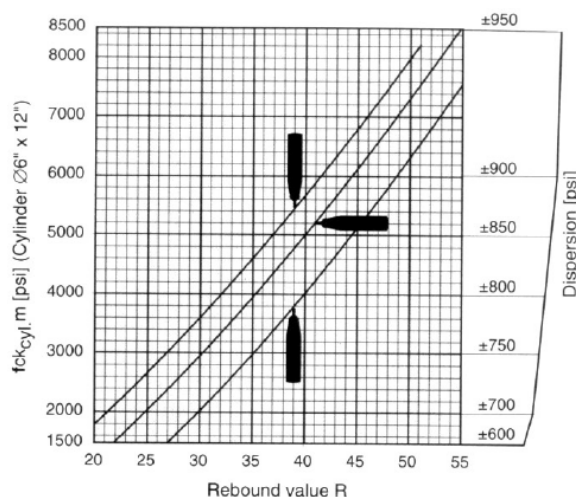
Figure 2.7 Conversion curves based on the average compressive strength of a cylinder and the rebound value of R .
