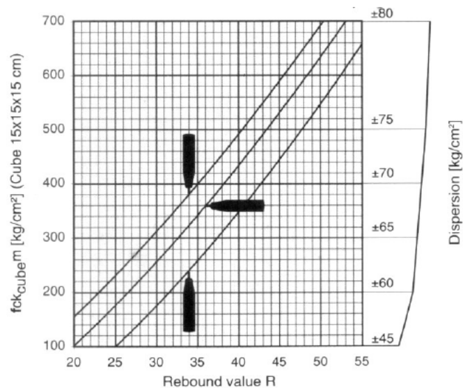
Figure 2.6 Conversion curves based on the average compressive strength of a cube and the rebound value R .
